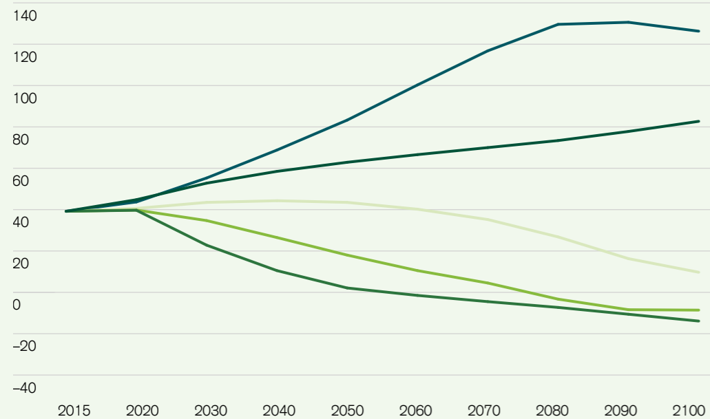
Figure 42: CO 2 emission profiles associated with IPCC global warming scenarios
